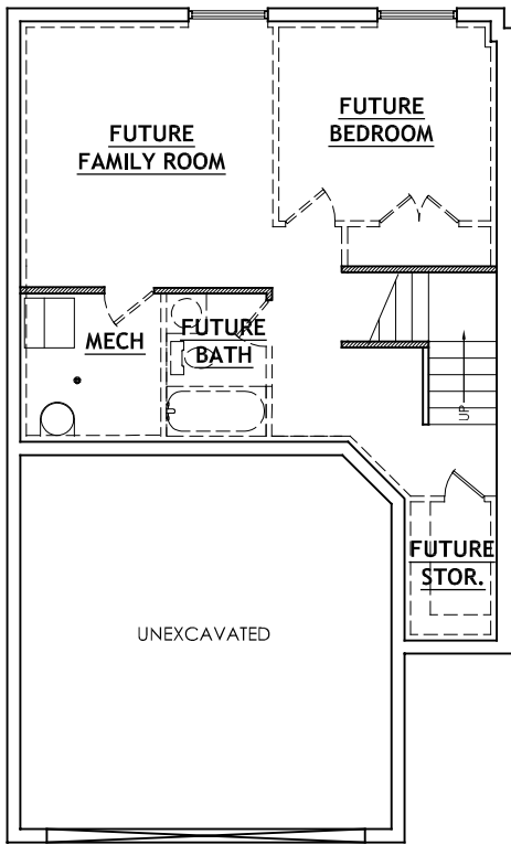
UNFINISHED BASEMENT
