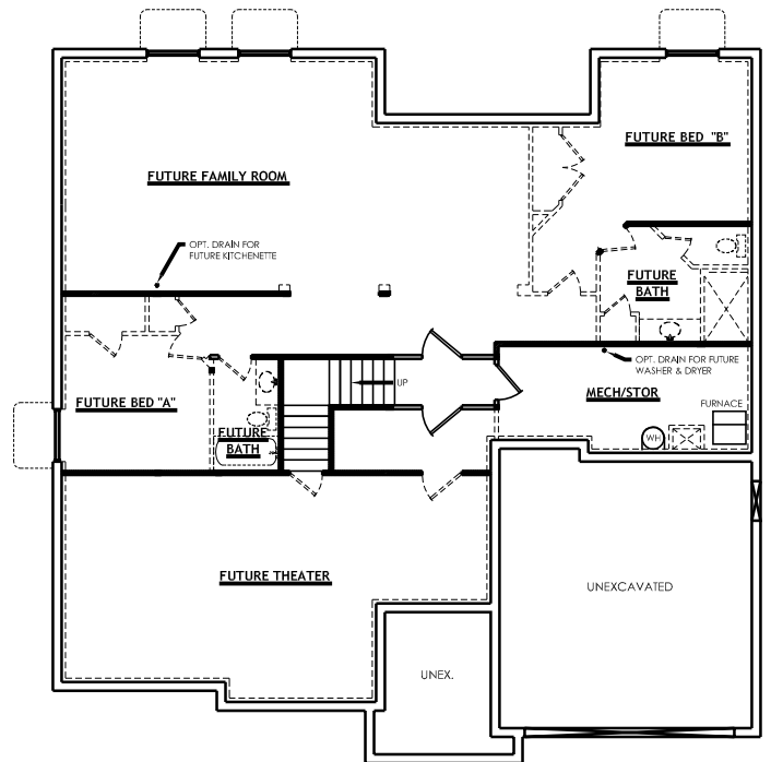
UNFINISHED BASEMENT (OPT. 9' WALLS)
