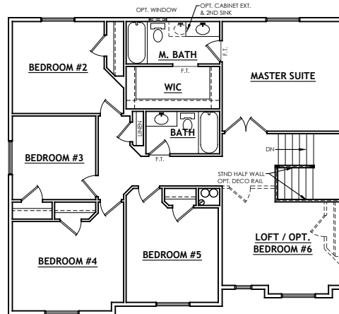
UPPER LEVEL (OPTIONAL 9'-0" CEILING)
