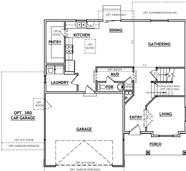
MAIN LEVEL (OPTIONAL 9'-0" CEILING)
