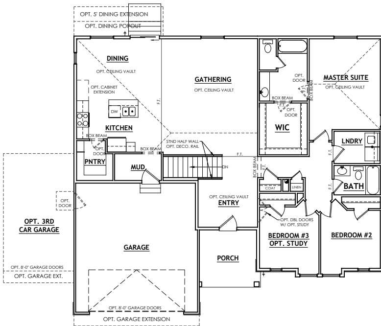
MAIN LEVEL (OPT. 9' CEILING)
