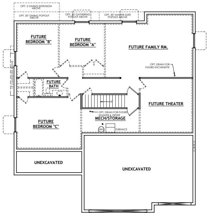
UNFINISHED BASEMENT (OPT. 9'-0" WALLS)
