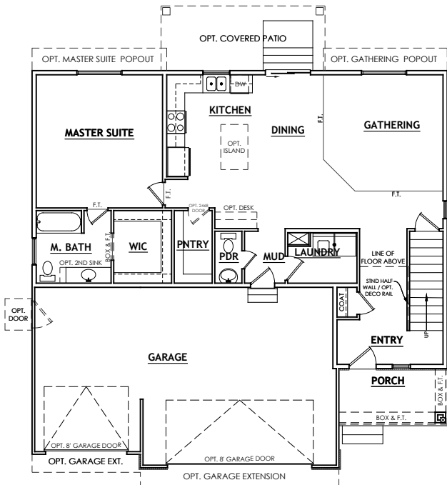
MAIN LEVEL (OPTIONAL 9'-0" CEILINGS)
